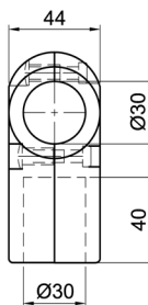
T-Verbinder, 2-schalig T-Connector, 2-shell
