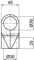
T-Verbinder, 2-schalig T-Connector, 2-shell
