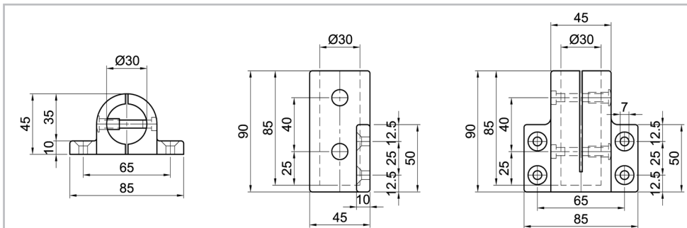
Wandlager, 1-schalig Wall bearing, 1-shell
