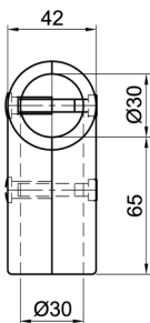
T-Verbinder, 2-schalig T-Connector, 2-shell
