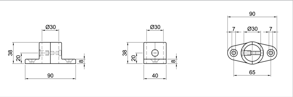
Bodenlager, 2-schalig Ground bearing, 2-shell
