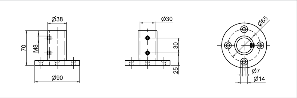
Bodenlager, 1-schalig Ground bearing, 1-shell
